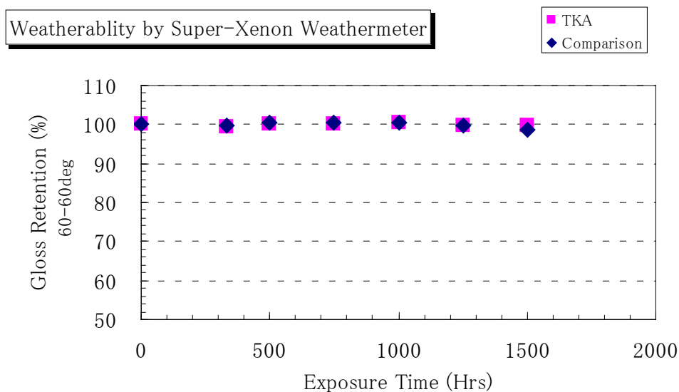
Fig-1. Weatherability of DURANATE™ TKA-100 with acrylic polyol Polyol: Acrylic A801 (supplier DIC Co., Ltd. )
